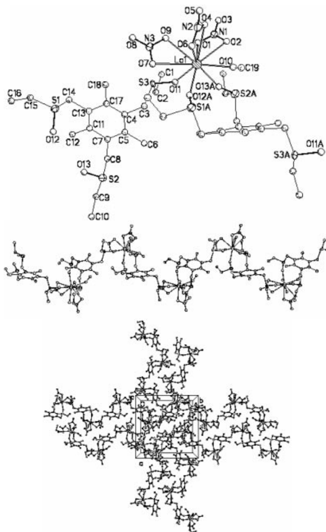
Figure 1. (Top) View of 1 showing the coordination environment of the center ion, (middle) the helical-chain structures of 1 (or 2 ) and (bottom) crystal packing diagram in 1 (or 2 ), only one position of the disordered sets of S atoms is shown
