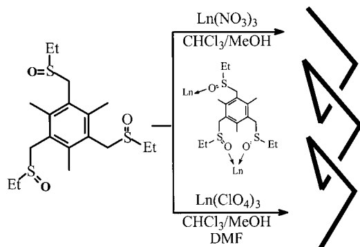
Scheme 1. Schematic representation of the formation of 1–3
