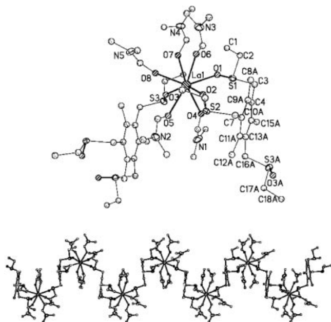
Figure 2. (Top) View of 3 showing the coordination environment of the center ion and (bottom) the helical-chain structure of 3 , only one position of the disordered sets of S atoms is shown
